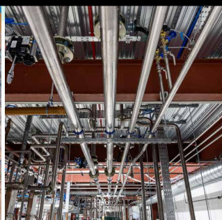
Hygienic/Service Pipework
